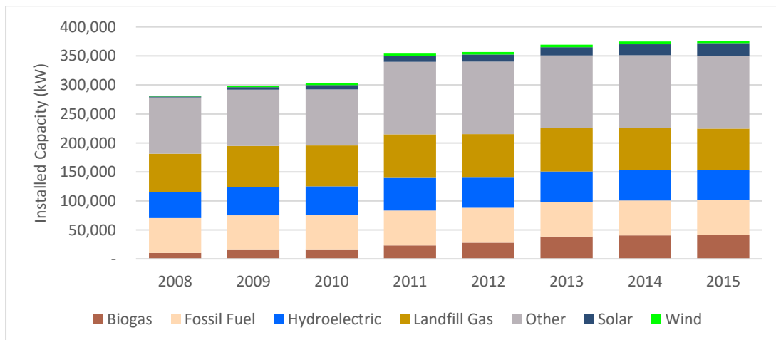
Figure 18: Cumulative Kilowatts of Installed DER Capacity, by Technology Type, 2008-2015
