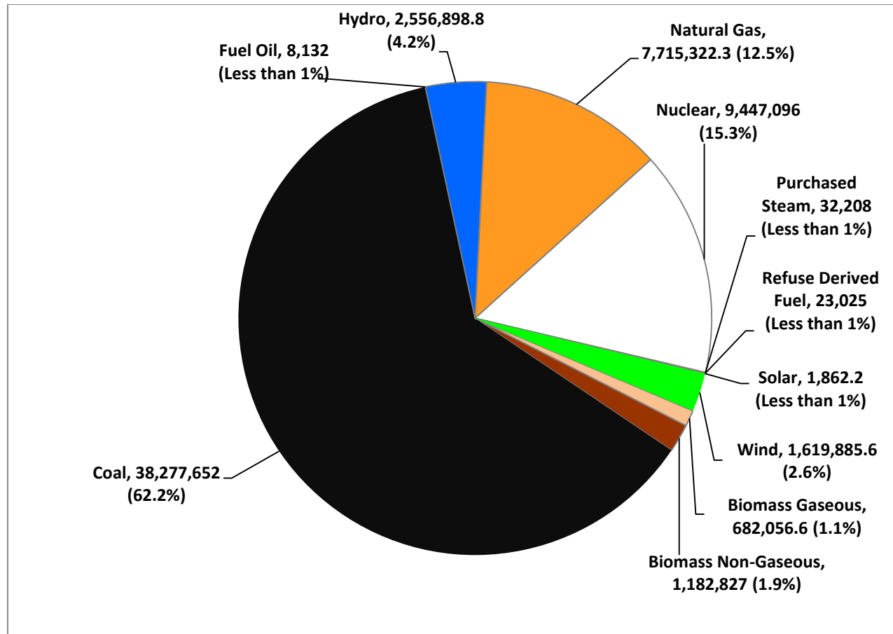
Figure 8: Wisconsin Electricity Generated by Fuel Source, 2014 (MWh)
